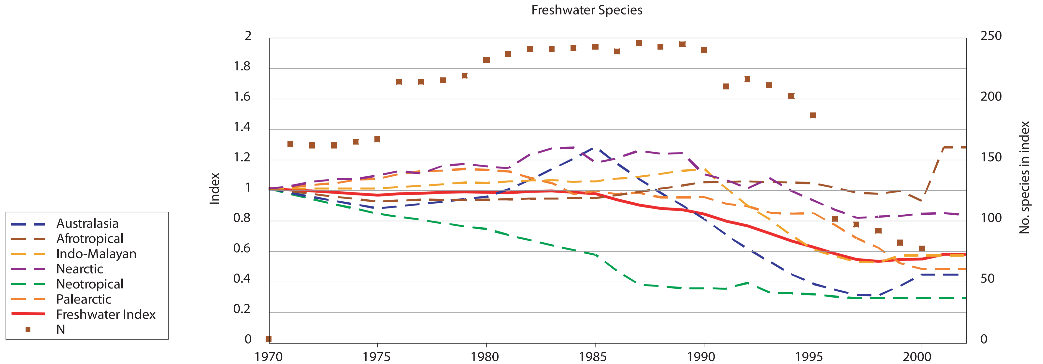
Figure 5.2: Living Planet Index, 1970-2000
